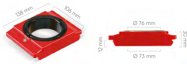
BOCCOLA HSK A100-B125
