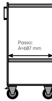
CARRELLI SMART 073
